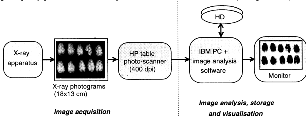
Fig. 1. Computer system for analysis of X-ray images of grains.
